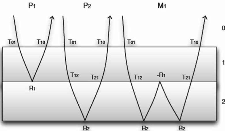
Fig. 3. A layered medium used for synthetic data modeling. The first layer, 0, is acoustic and the deeper two are anelastic. Three events are depicted with the coefficients that alter their amplitudes. The parameters used in forward modeling are displayed in Table 1.
