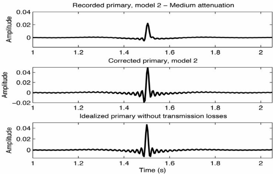
Fig. 11. A comparison of the actual primary (top curve), the corrected primary (middle curve) and the idealized primary, generated without transmission losses (bottom curve) for model 2, the medium attenuation case.
