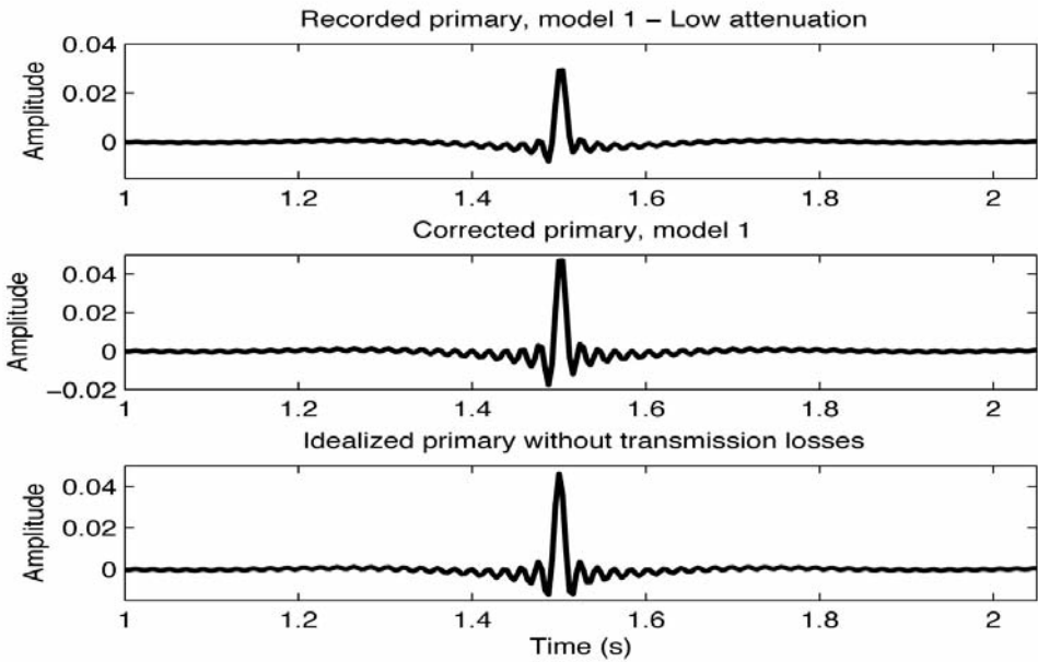
Fig. 10. A comparison of the actual primary (top curve), the corrected primary (middle curve) and the idealized primary, generated without transmission losses (bottom curve) for model 1, the low attenuation case.
