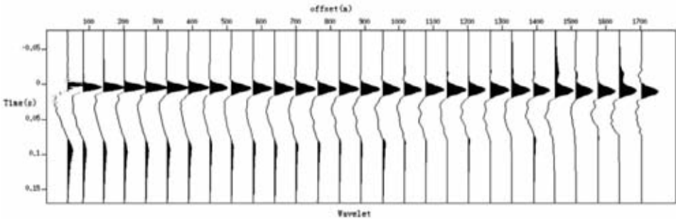
Fig. 19. Wavelet A(t), cable II (source at depth 7 m and receivers at depth 18 m).
