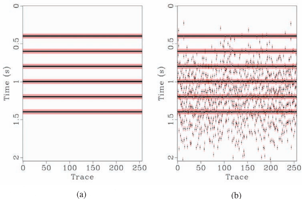
Fig. 3. First synthetic example (sorted to common offset domain). (a) Unblended data. (b) Blended data.
