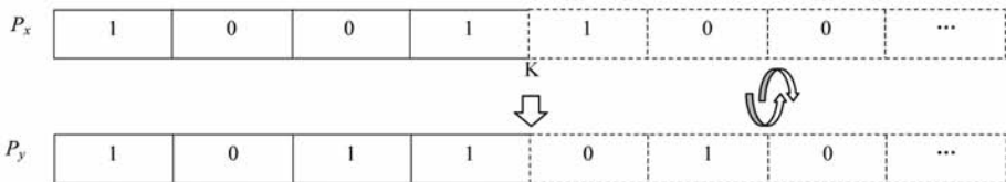
Fig. 2. Crossover operation diagram of GA inversion. P_x and P_y are two individuals randomly selected in the population. Since the K value is usually relatively small, the exchange of the encoding parameters after the encoding bit K is equivalent to the optimization operation in the vicinity of the solution.
