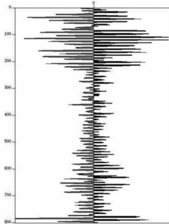
Fig. 8. The convolution of the wavelet in Fig. 3 with the reflectivity in Fig. 6 produces the above trace.
