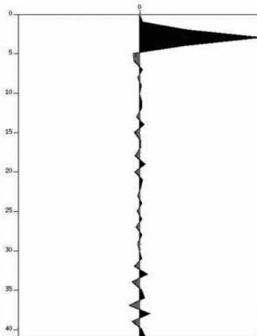
Fig. 6. The application of a Wiener deconvolution spiking filter (length = 5, prewhitening = 1% ) to the shaped wavelet of Fig. 5 (a cascaded deconvolution) produces a resolving kernel that more closely resembles a spike than the direct deconvolution resolving kernel of Fig. 4.
