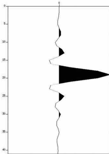
Fig. 4. The output from applying a Wiener spiking filter to the wavelet in Fig.3.
