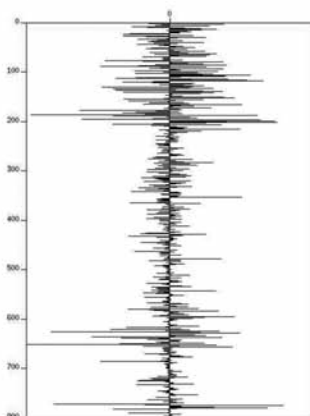
Fig. 7. The reflectivity function used in Dey (1999), as derived from well logs of a central Alberta well.
