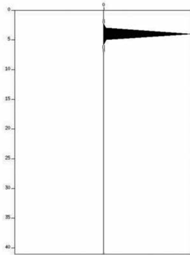
Fig. 2. Filter output from application of a Wiener spiking filter converts the exponentially damped sinusoid wavelet in Fig. 1 to a nearly perfect spike as anticipated by previous analysis in eqs. (1)-(5).
