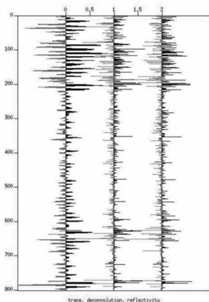
Fig. 10. A comparison of an input trace (left trace) with the cascade deconvolution (middle trace) and the actual reflectivity. The deconvolution correlates very well with the desired reflectivity function.
