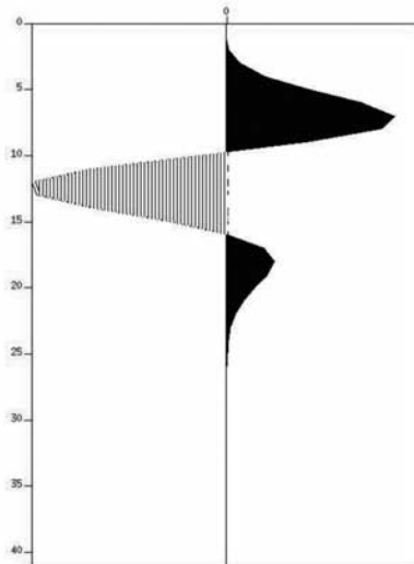
Fig. 3. A seismic wavelet as used in Dey (1999).
