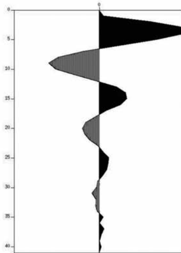
Fig. 5. The output from applying the shaping filter of eq. (7) to shape the wavelet of Fig.3 to the wavelet of Fig. 1.
