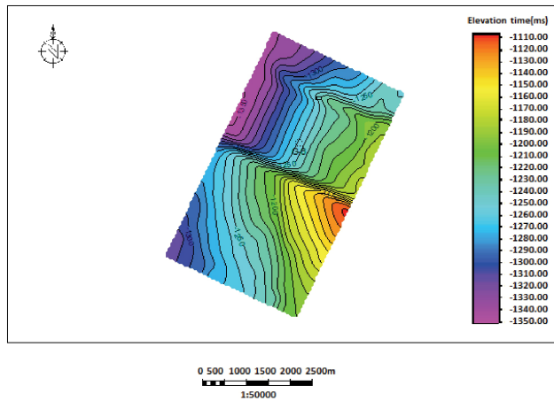
Fig. 3. Structural contour map shows the top part of Pariwar Formation in the study area. (Khan and Khan, 2015).
