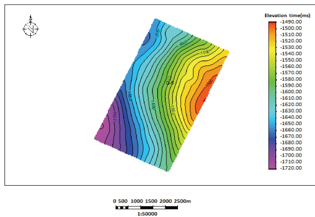
Fig. 4. Structural contour map shows the bottom part of the Pariwar Formation in the study area.
