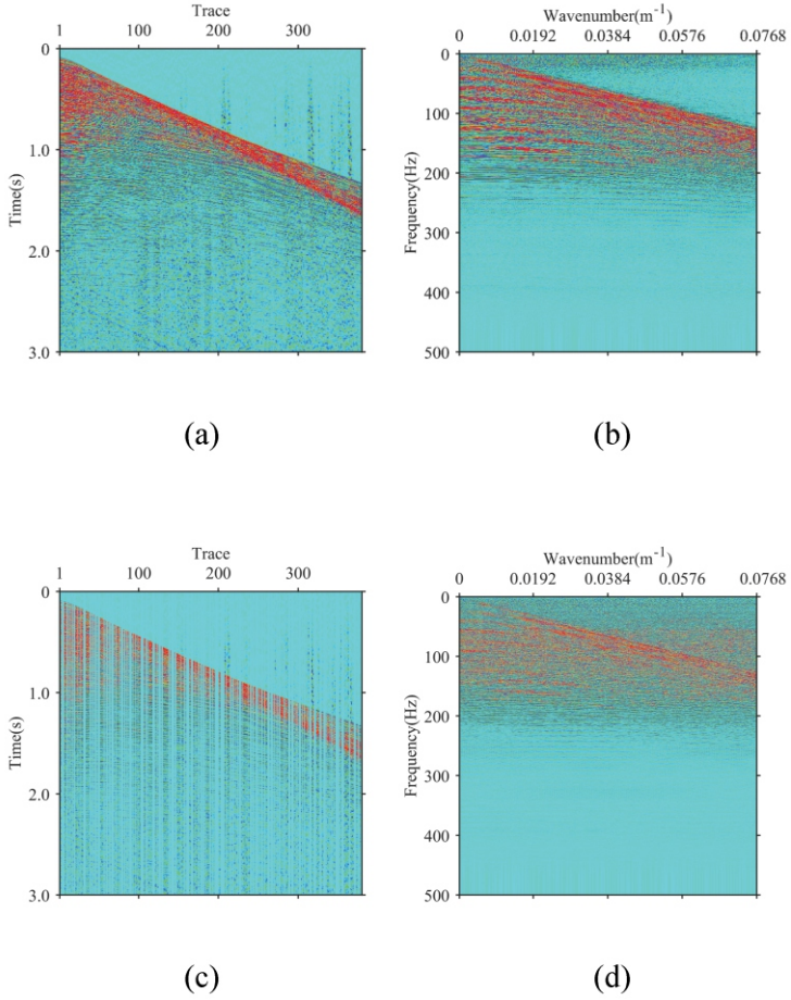
Fig. 7. (a) Field data, (b) 2D-DCT of (a), (c) 30% random decimated of (a), (d) 2D-DCT of (c).
