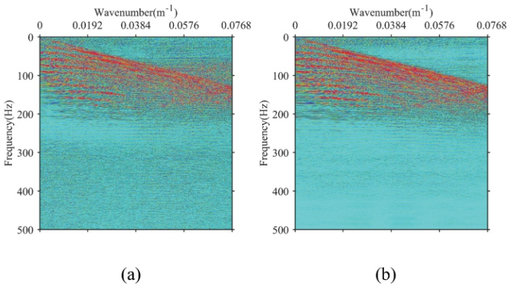
Fig. 9. DCT data comparison (a) DCT of Fig. 8 (a) reconstructed in shearlet domain, (b) DCT of Fig. 8 (c) reconstructed in DCT+shearlet domain.
